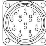
12 Pin SSI
