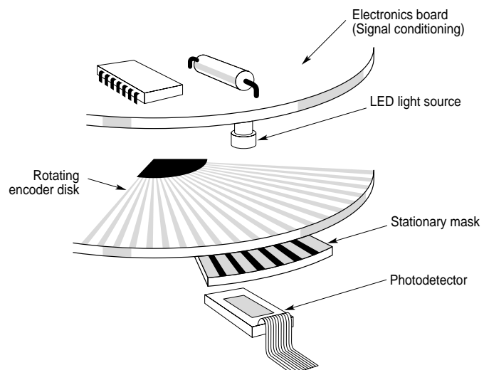
The basic structure of an incremental encoder with conventional code disk.
